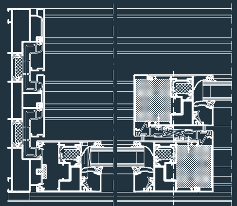
Schüco Hebe-Schiebesystem ASS 70.HI, M = 1:5 Schüco lift-and-slide system ASS 70.HI, scale = 1:5
